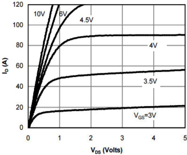
Output Characteristic
