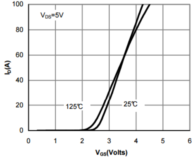
Transfer Characteristic
