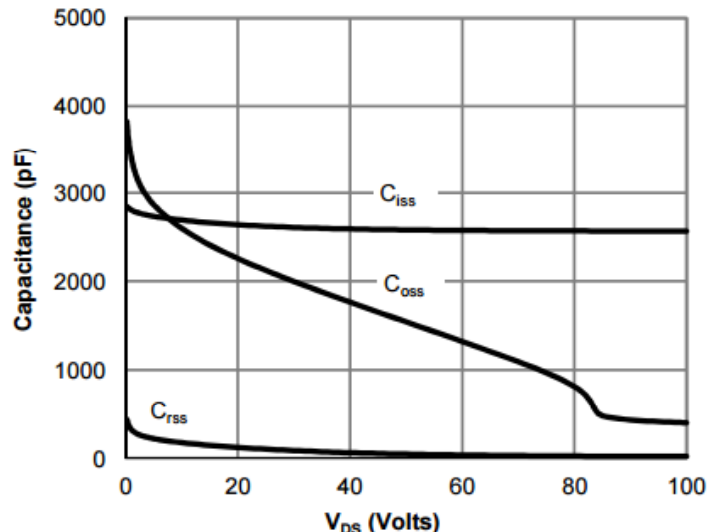
Capacitance
